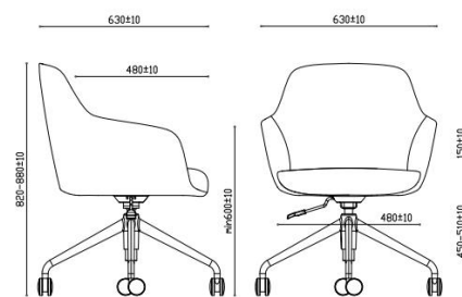
L7102 Swivel base version
